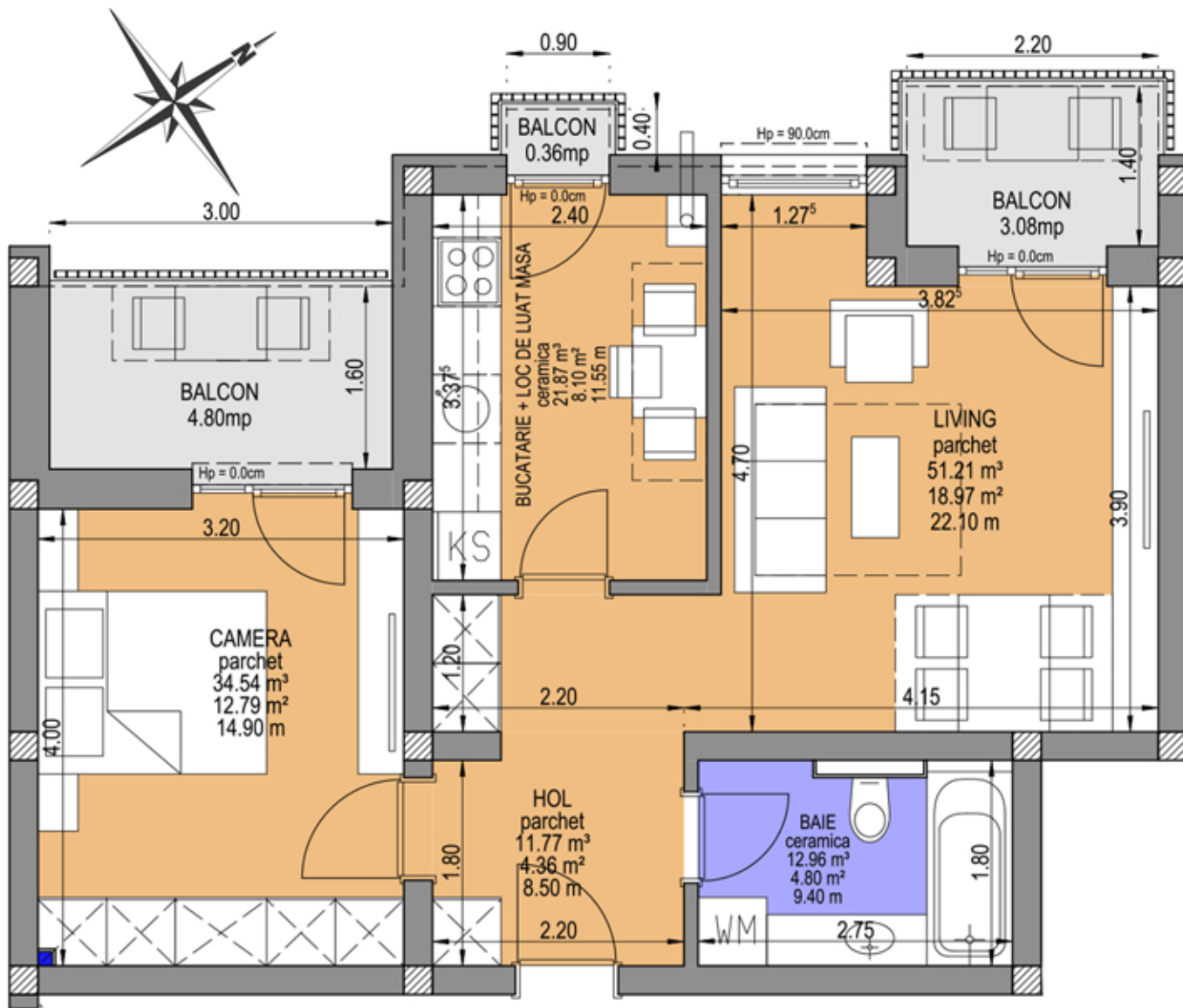
AP. 2 CAMERE - TIP STUDIO 49.03mp (AP. 204)
